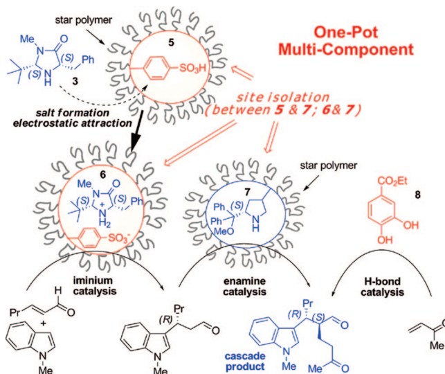
Figure 1. Illustration of our design: non-interpenetrating star polymers for one-pot cascade catalysis.
