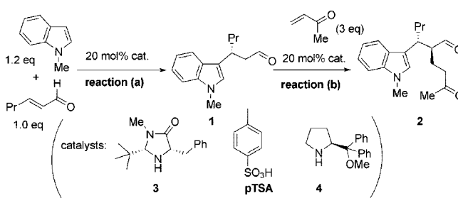
Scheme 1. Study of Each Individual Reaction Step Using Small Molecule Catalysts
